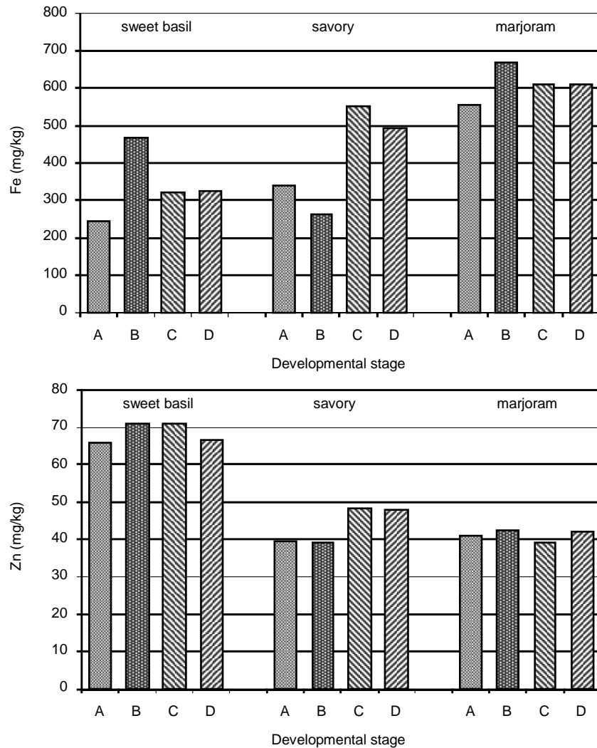
Fig. 1. Iron and zinc content in the raw material of the selected herbal plants depending on developmental stage of plants: A – vegetative stage, B – beginning of flowering, C – full flowering, D – seed setting
